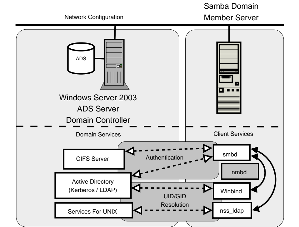
Figure 7.3 Active Directory Domain: Samba Member Server
